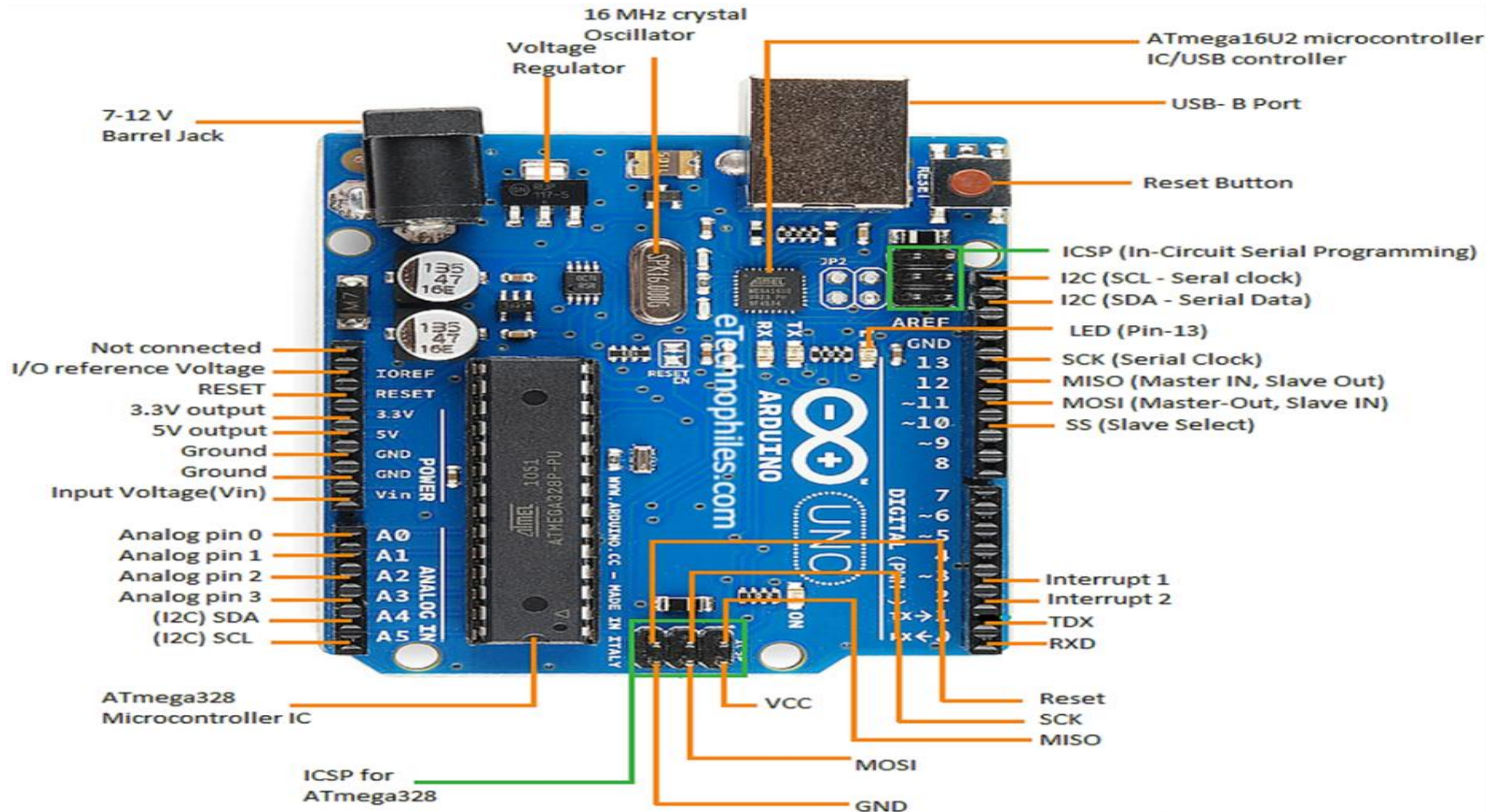
A basic Arduino Uno board
